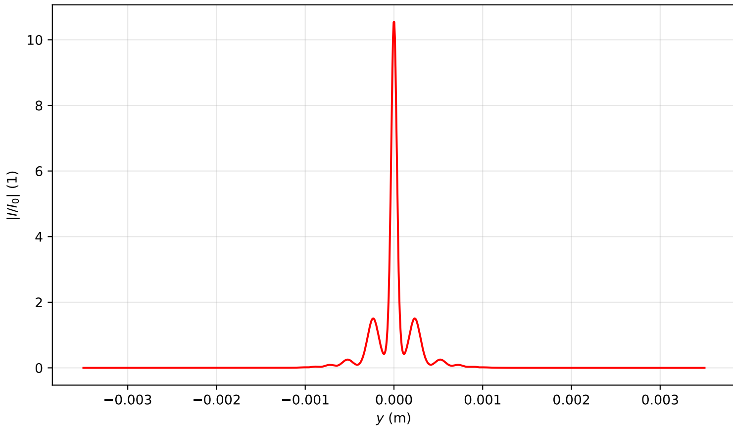
Intensity profile I(x=0, y, z=0.478)/I_0 , P_{in}=8.5P_{cr} , artificial time
